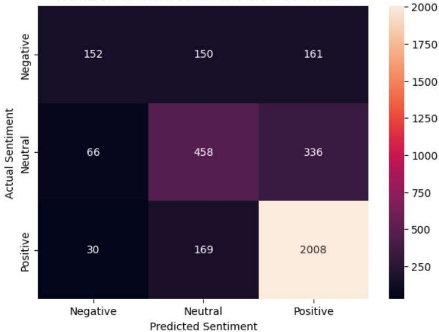
YouTube Comment Sentiment Confusion Matrix
